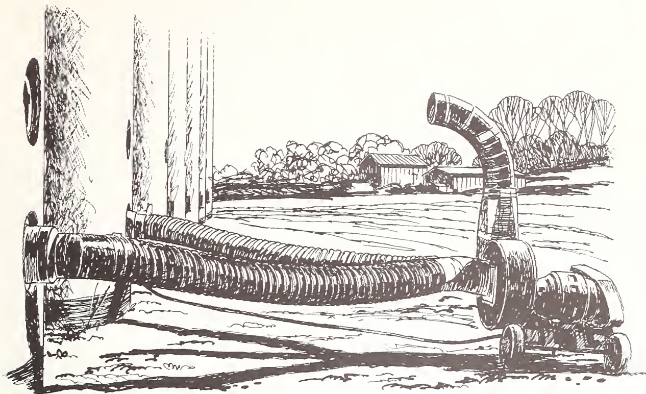
FIGURE 11.—Connections made to evacuate the fumigant simultaneously from both tanks.
